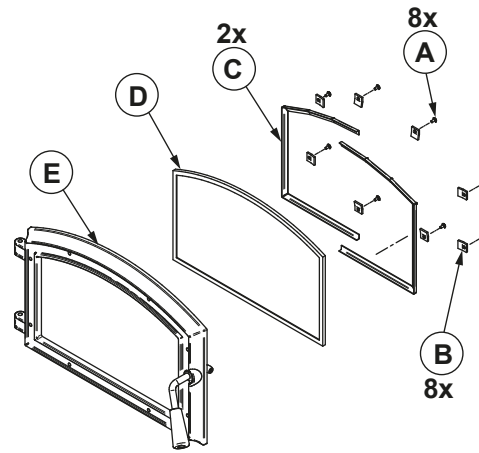
Figure 22 : Replacing the glass
